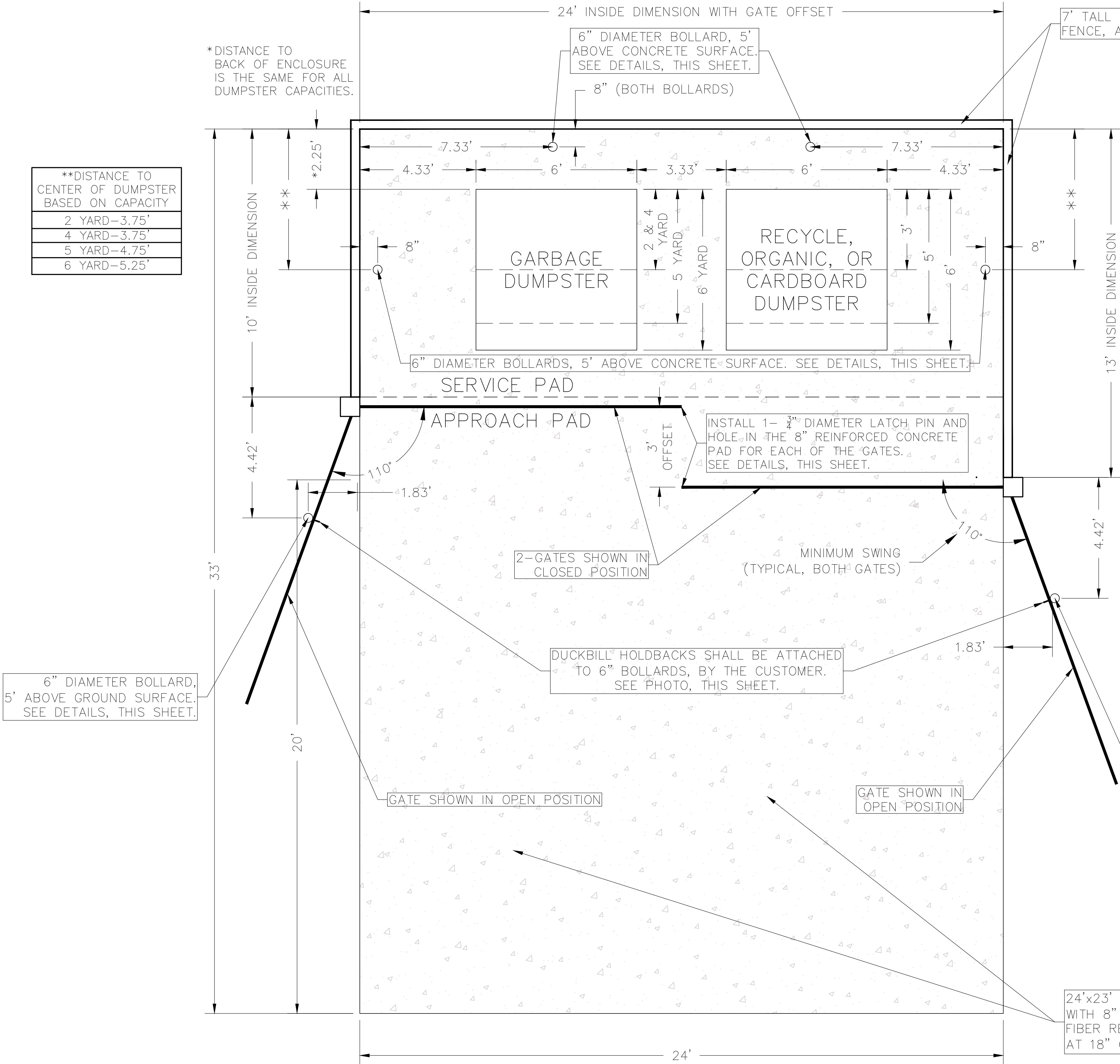
REAR LOAD CONTAINER ENCLOSURE LAYOUT PLAN
