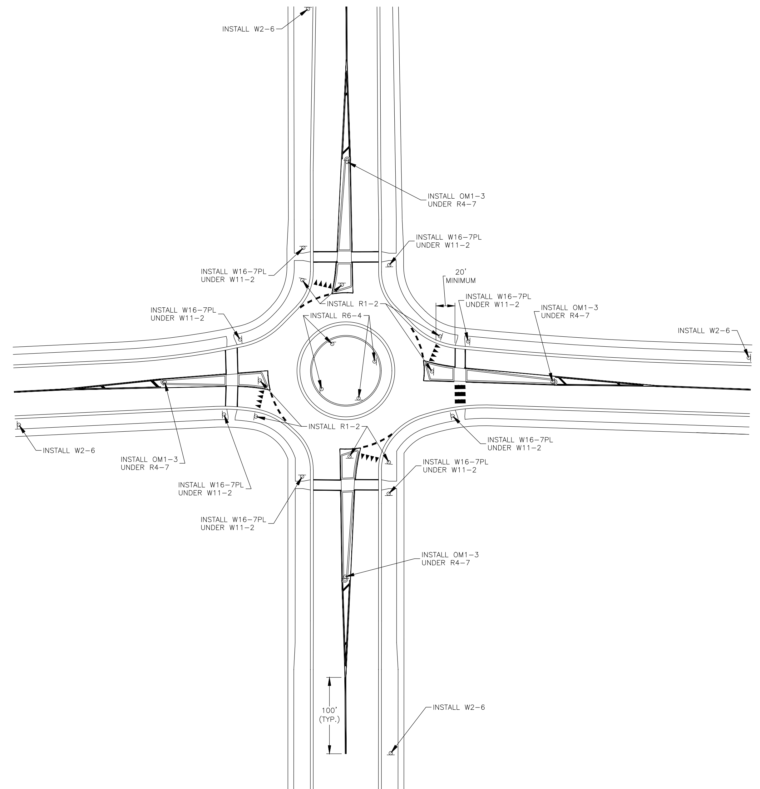
TYPICAL ONE-LANE ROUNDABOUT SIGNING DETAILS
