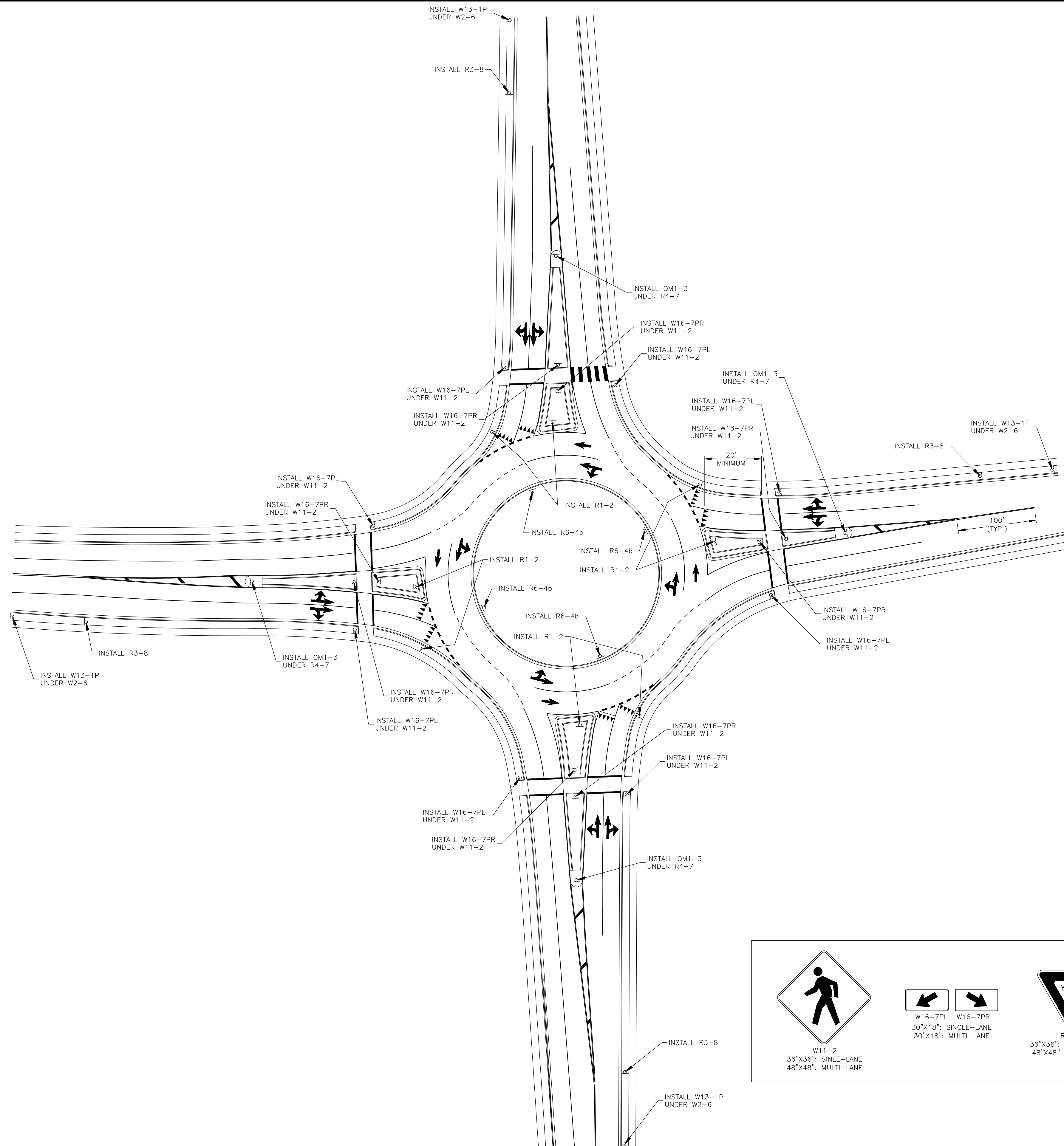
TYPICAL TWO-LANE ROUNDABOUT SIGNING DETAILS
