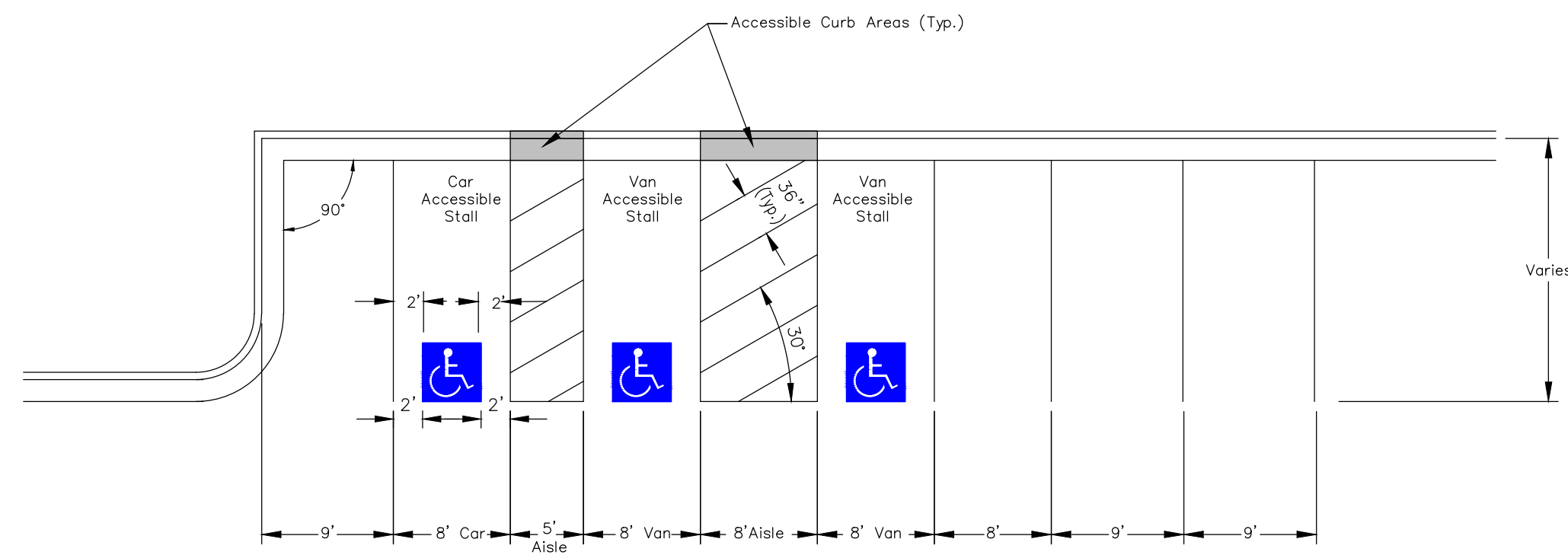
90 DEGREE ANGLE PARKING
