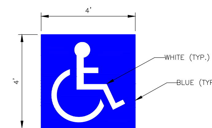
INTERNATIONAL SYMBOL OF ACCESSIBILITY
