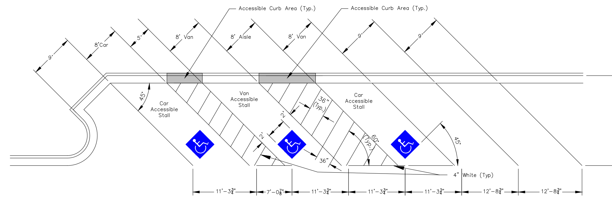
45 DEGREE ANGLE PARKING
