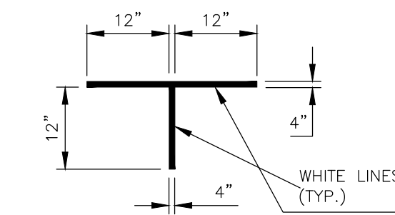
ON-STREET PARKING STALL PAVEMENT MARKING (TEE)
