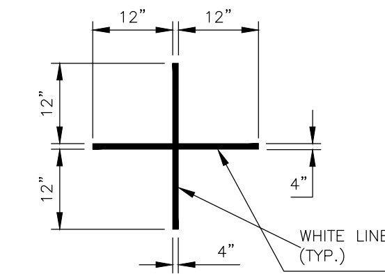
ON-STREET PARKING STALL PAVEMENT MARKING (CROSS)
