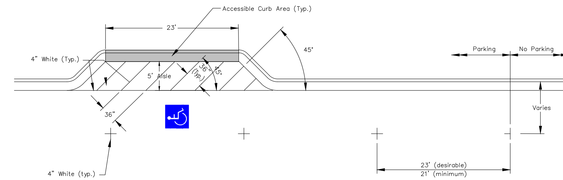
PARALLEL PARKING SPACE PAVEMENT MARKING
