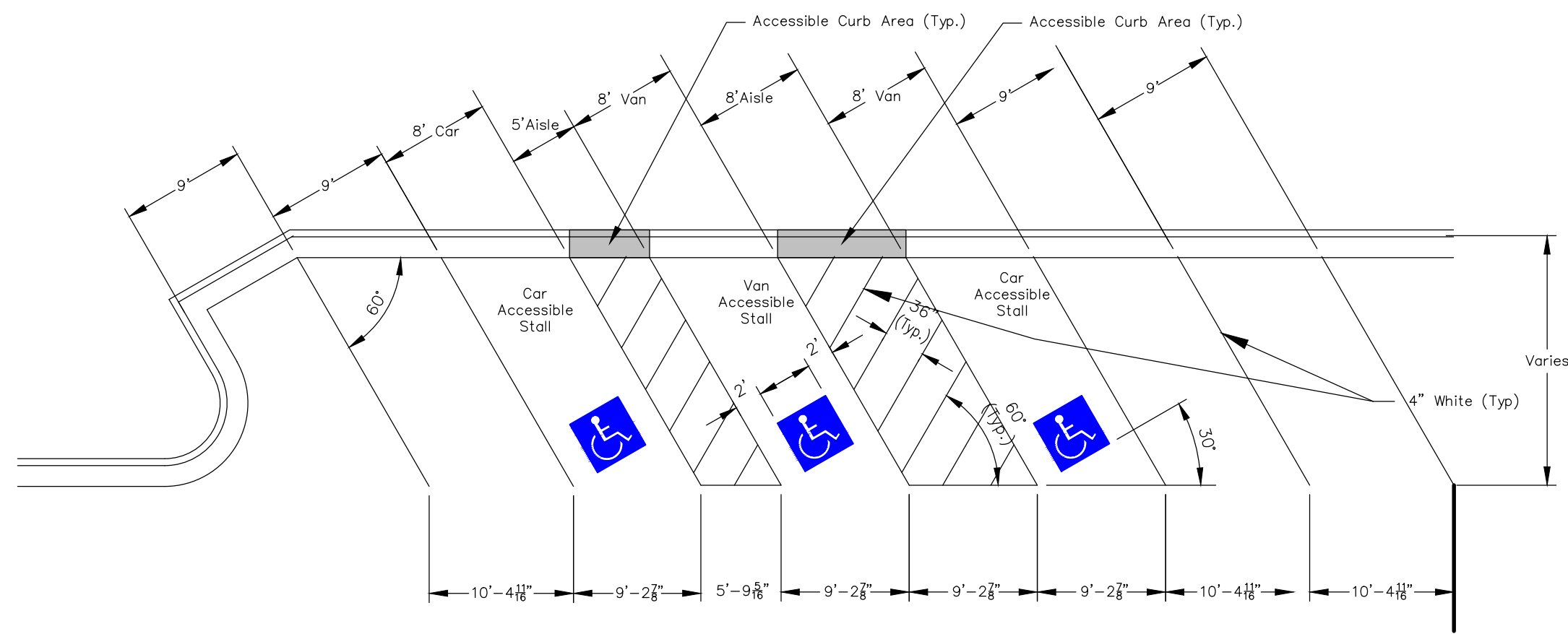
60 DEGREE ANGLE PARKING
