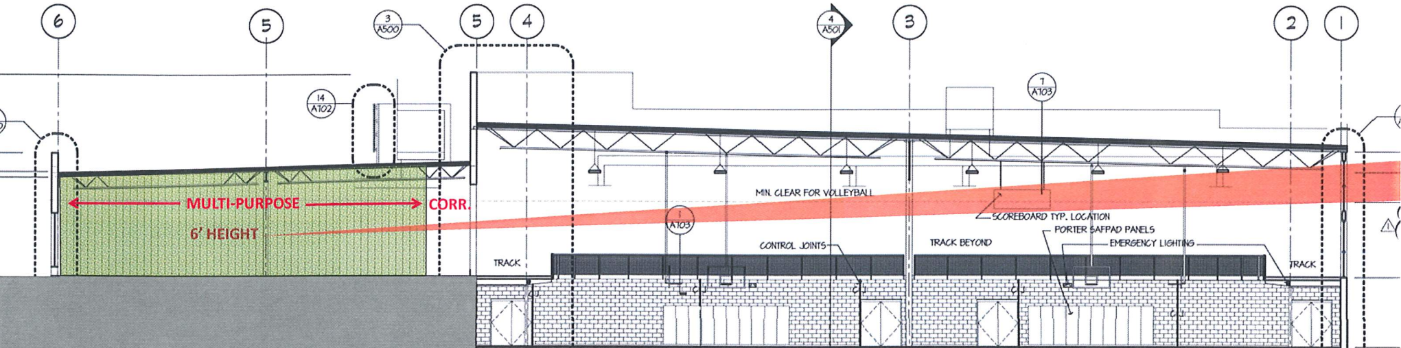
SECTION THROUGH MULTI- PURPOSE AND GYM
