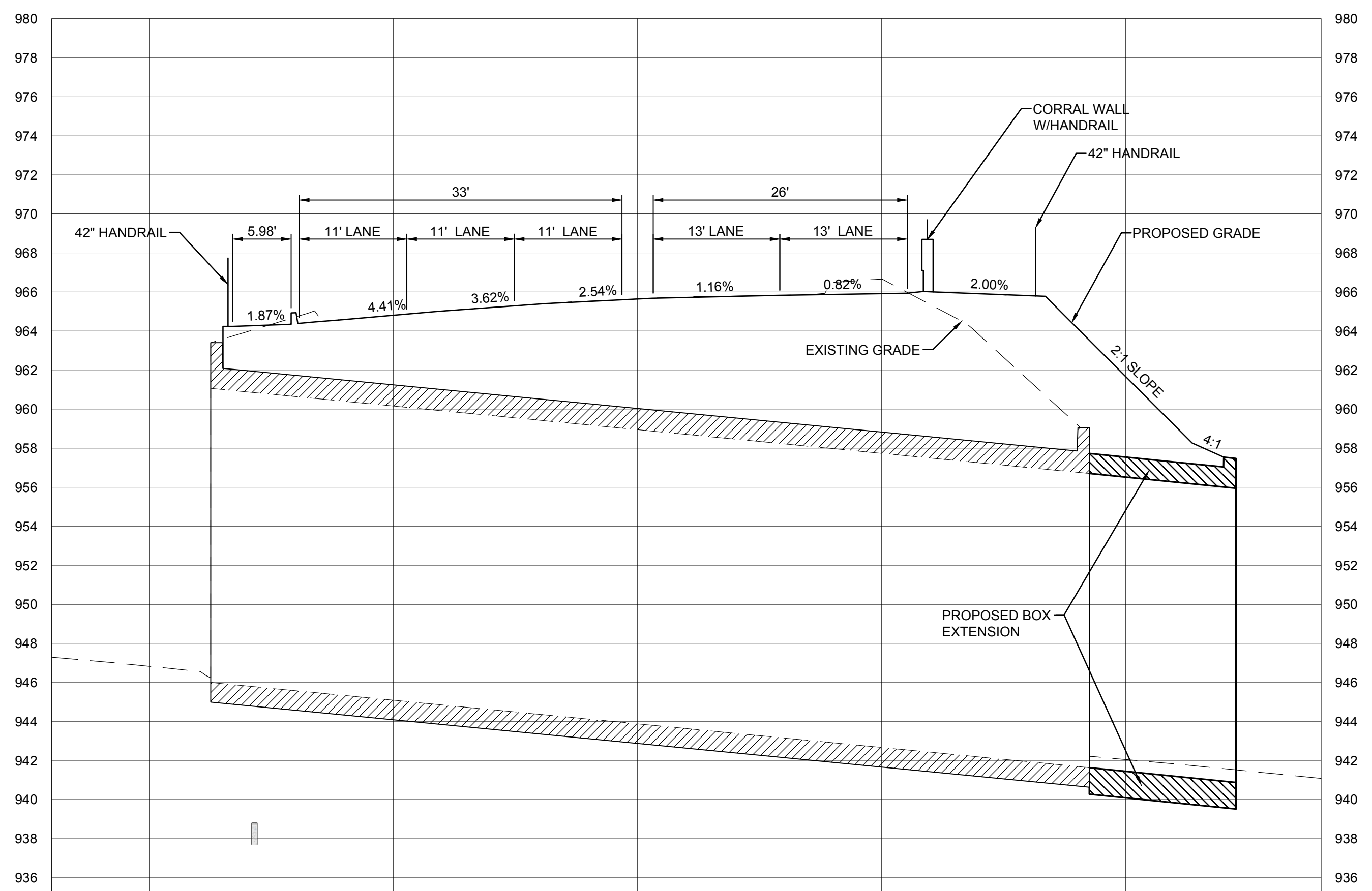
SECTION A-A HORIZONTAL 1" = 10' VERTICAL 1" = 5'
