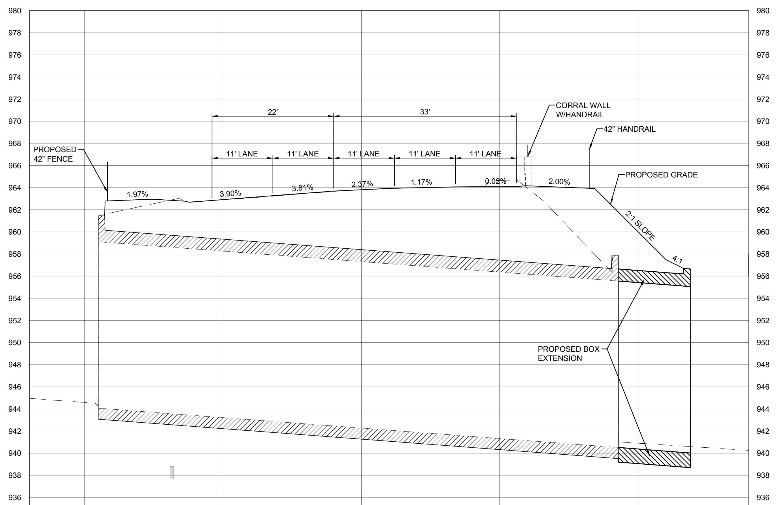
SECTION B-B HORIZONTAL 1" = 10' VERTICAL 1" = 5'
