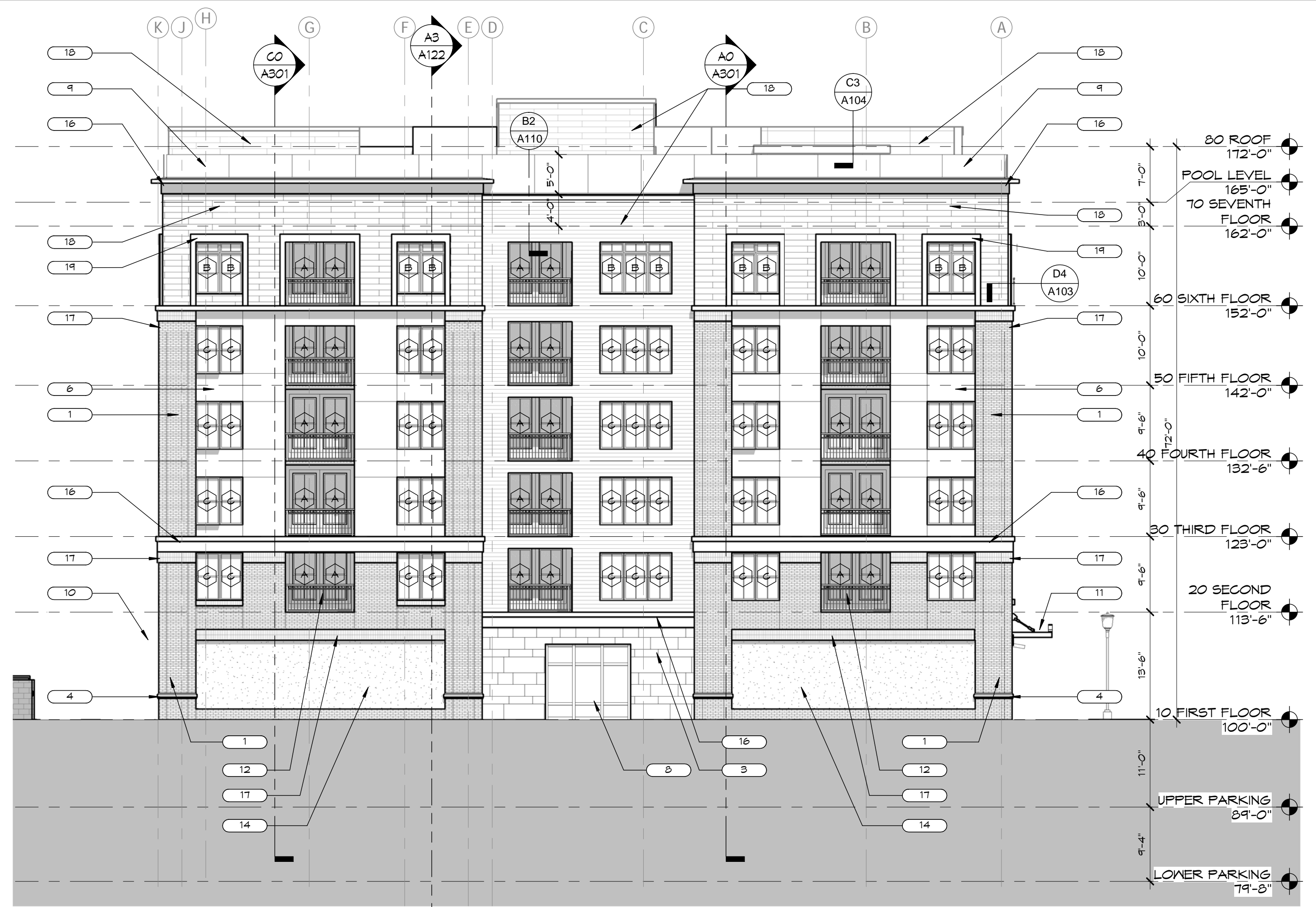
NORTH ELEVATION A1
