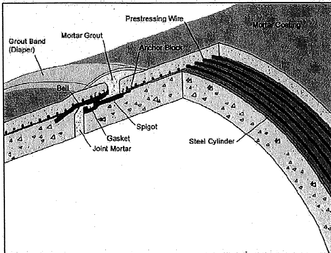
Typical Cross-Section of Prestressed Concrete Cylinder Pipe
