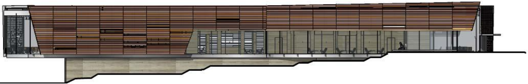
SOUTH ELEVATION
