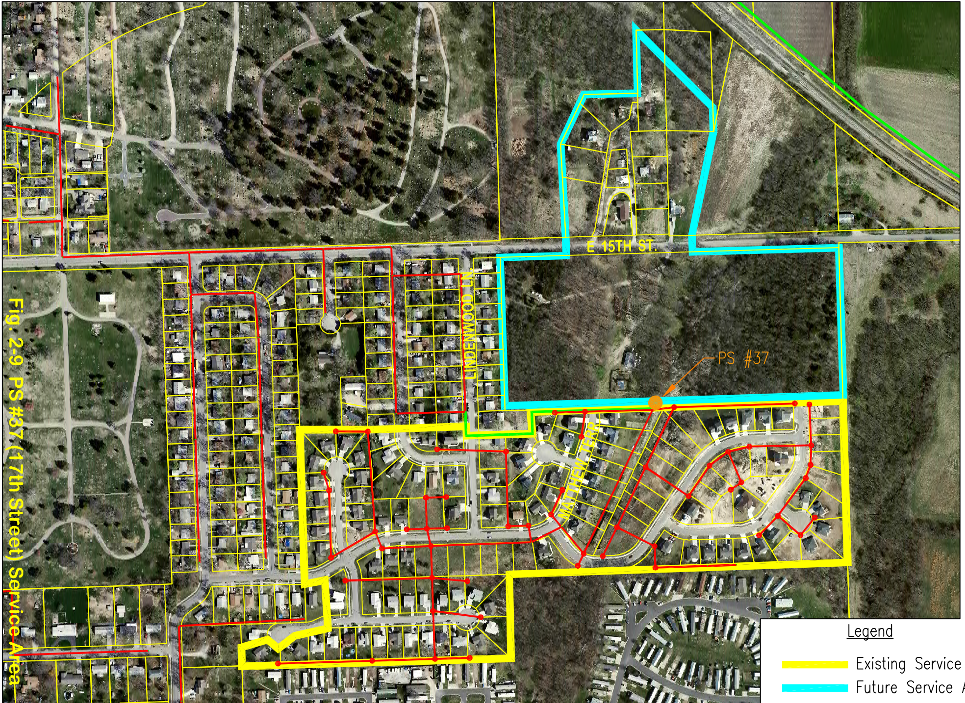
Figure 2-9 PS#37 (17th Street) Service Area
