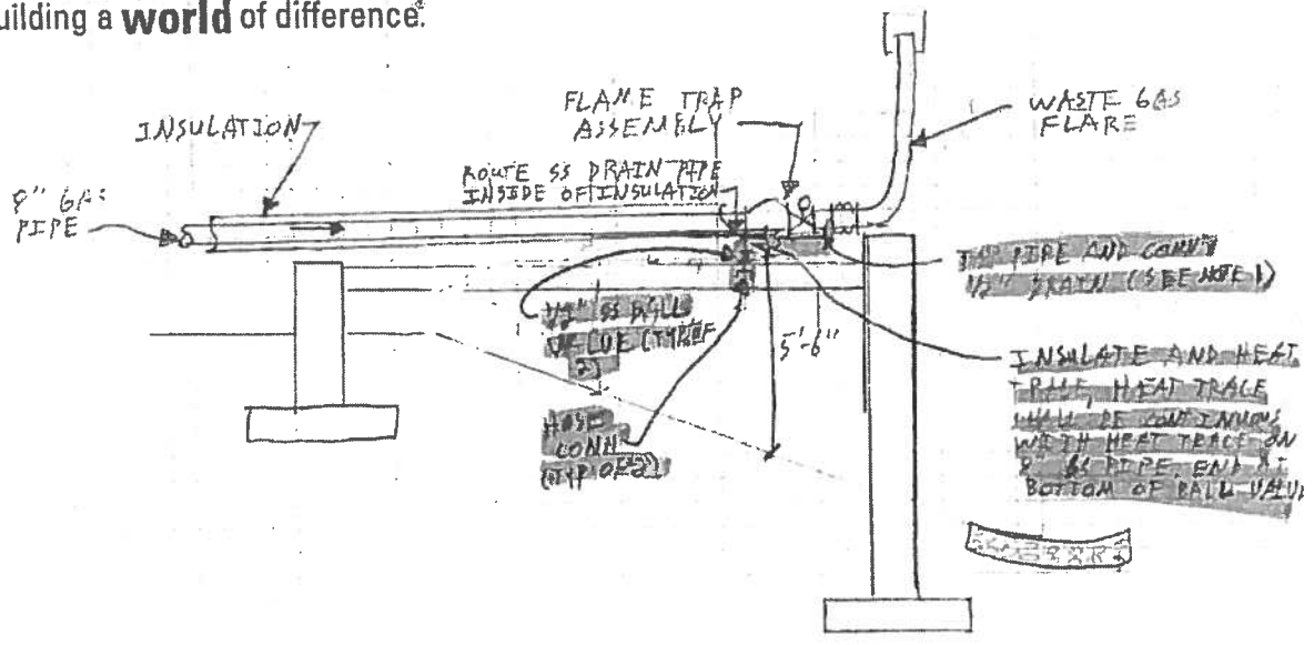
sketch of adding drain to Flame Trap assembly at Waste Gas Flare
